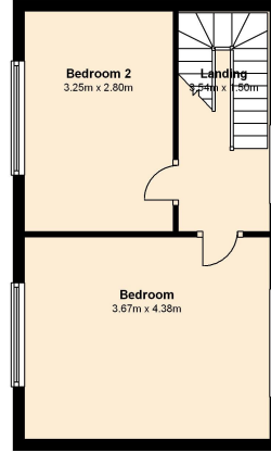
Second Floor Approx. 30.4 sq. metres
