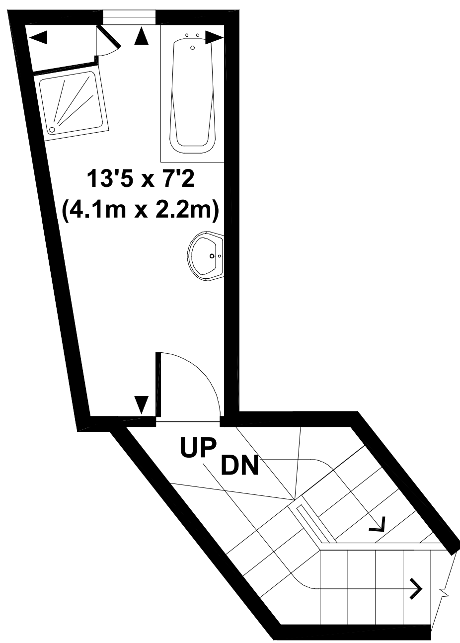
GROUND FLOOR / HALF LANDING
